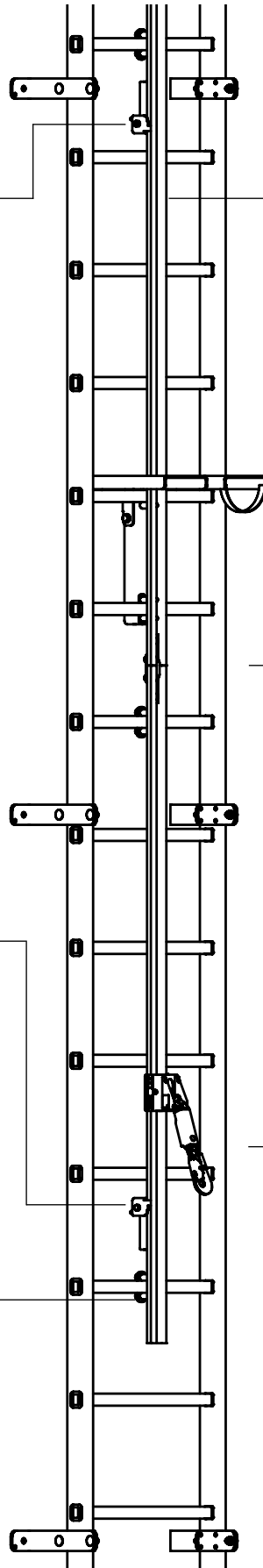
H-50 Endanschlag/ H-50 end stop
